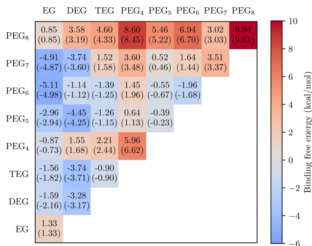
Fig. 4 Cluster binding free energies for (PEG n )(PEG m )-dimers up to n, m = 8 . The lowest formation free energy minima are accompanied in brackets with the values Boltzmann averaged over a set of low lying free energy configurations. Temperature is 298.15 K and reference pressure 1 atm.
