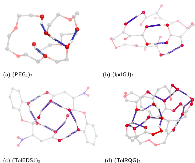
Fig. 2 Some examples of lowest free energy cluster configurations, with hydrogen bonds highlighted in blue. Note that hydrogens bonded to carbons have been omitted.
