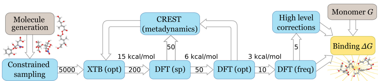
Fig. 1 Configurational sampling workflow used in this paper. Filters (arrows) are applied between each computational step. The filtering thresholds E_{\text{lim}} are shown above the arrows, and the maximum number ( N_{\text{lim}} ) configurations passed to the next step is shown inside each arrow. High level corrections may involve a single-point calculation, or re-optimization of the structure.
