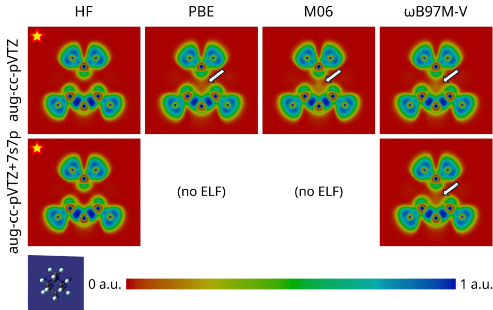
Fig. 5 Isocontour plots of the anionic ELF at the equilibrium geometry of neutral C_{10}F_{16} , for different methods and basis sets (specified in the figure). The ELF were plotted in a plane through the center of the molecule and containing four carbon atoms (see the inset at bottom left). Stars indicate results for vertically unbound anions obtained using charge stabilization, and the arrows indicate the very weak localization in the cage center.
