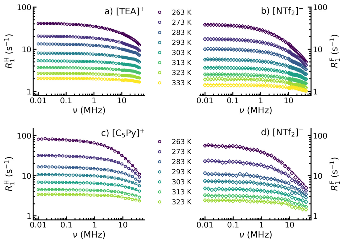
Fig. 2 Temperature dependent NMRD profiles for ^1H (a) and (c) plotted as circles and ^{19}F (b) and (d) plotted as diamonds in the ionic liquids [TEA][NTf _2 ] (a) and (b) and [C _5 Py][NTf _2 ] (c) and (d). The solid lines correspond to the model fits according to eqn (1), (5), (9) and (12) for [TEA][NTf _2 ] as well as to eqn (1), (6), (9) and (12) for [C _5 Py][NTf _2 ].
