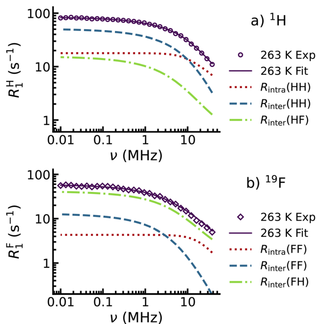
Fig. 3 Dissected NMRD profiles at 263 K for (a) ^1H and (b) ^{19}F in the IL [C _5 Py][NTf _2 ]. Experimental data are plotted as open symbols, while the total fits are shown as purple solid lines. The contributions from homonuclear intermolecular relaxation R_{inter} are shown as blue dashed lines, heteronuclear intermolecular contributions R_{inter} as green dash dotted lines, and homonuclear intramolecular contributions R_{intra} are represented as red dotted lines.
