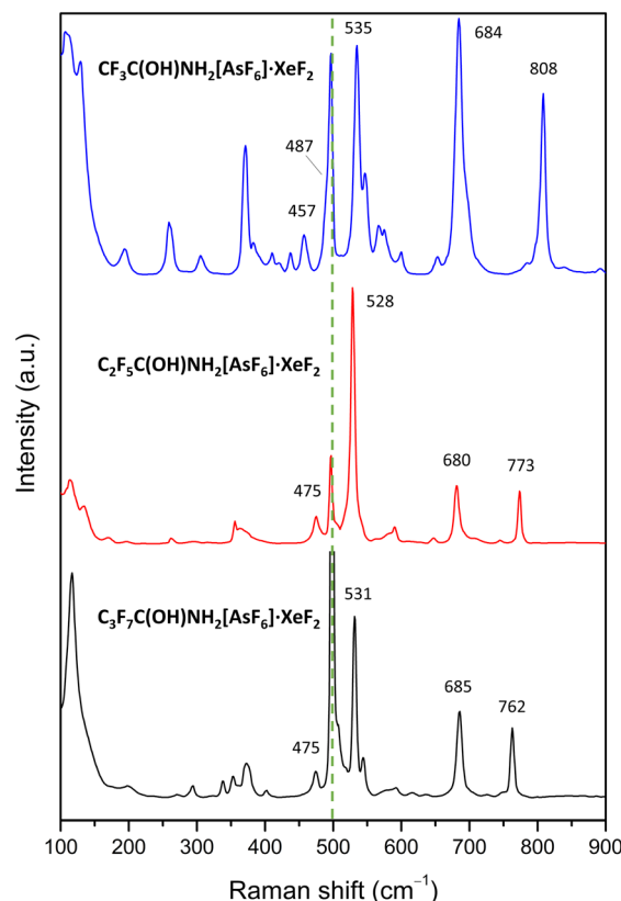
Fig. 8 Raman spectra of \text{XeF}_2 salt cococrystals with protonated amides recorded at low temperatures ( -90^\circ\text{C} ). The green dashed line is placed at the position of free \text{XeF}_2 ( 497\text{ cm}^{-1} ) 41 which was observed as an impurity in the reactions.
