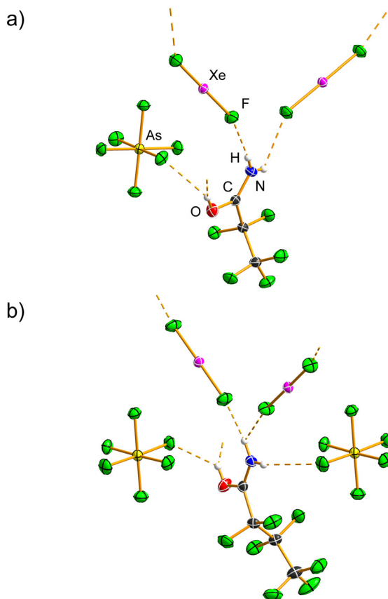
Fig. 7 Hydrogen bonds (dashed orange lines) in the crystal structures of the salt cococrystals (a) \text{C}_2\text{F}_5\text{C}(\text{OH})\text{NH}_2[\text{AsF}_6]\cdot\text{XeF}_2 and (b) \text{C}_3\text{F}_7\text{C}(\text{OH})\text{NH}_2[\text{AsF}_6]\cdot\text{XeF}_2 . The OH groups are bifurcated hydrogen-bond donors; however, two [\text{AsF}_6]^- anions have been omitted for clarity. Displacement ellipsoids are drawn at the 50% probability level, and hydrogen atoms are represented as spheres of arbitrary radius.
