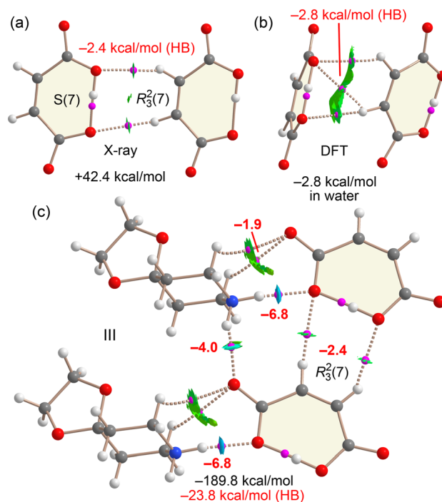
Fig. 23 QTAIM (BCPs in pink and bond path as dashed bonds) and NCiplot ( \text{RDG} = 0.5 , \rho cut-off = 0.04 \text{ a.u.} , color scale -0.035 \text{ a.u.} \leq (\text{sign} \lambda_2) \rho \leq 0.035 \text{ a.u.} ) for the H-bonded anion \cdots anion dimer in the X-ray (a) and optimized (b) geometries. (c) QTAIM analysis of a tetrameric fragment of III. The energies of the assemblies and those derived from potential energy densities (in red) are indicated in \text{kcal mol}^{-1} .
