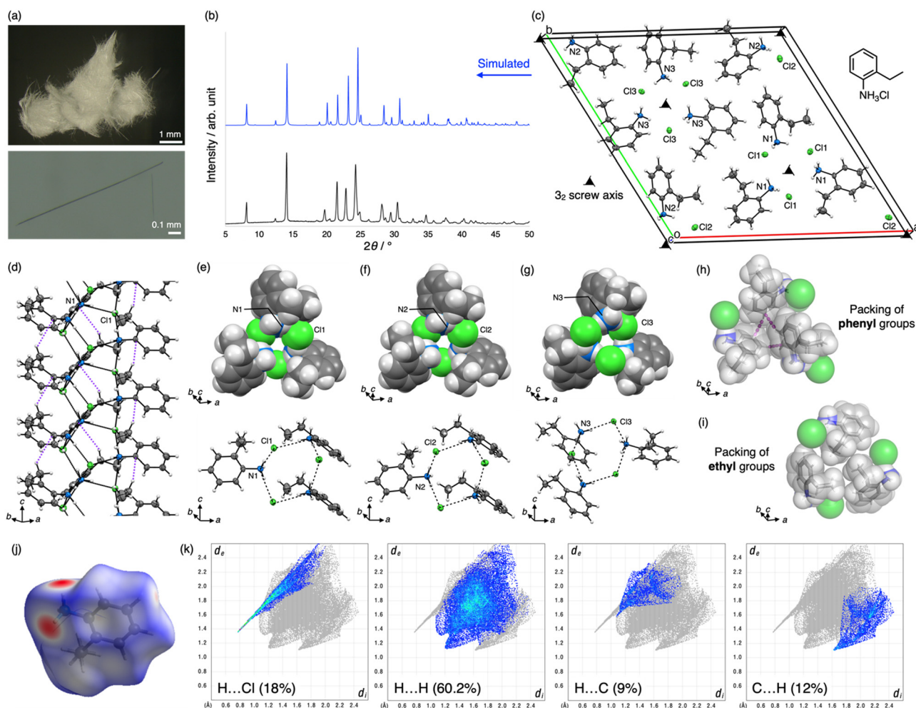
Fig. 2 Helical ammonium halide framework of 1 . (a) Photographs of the fibrous crystals of 1 . (b) PXRD pattern (CuK \alpha , rt) of the fibrous crystals (bottom) and a simulated pattern of the helical framework structure determined by ScXRD (top). (c) Unit-cell structure of 1 . (d) Side view of a helix composed of 2-ethylanilinium moieties with N1 and Cl1 atoms. (e)–(g) Top view of the helices and hexagonal hydrogen bonding units composed of N1 and Cl1, N2 and Cl2, and N3 and Cl3 atoms. (h) and (i) Packing structures of phenyl or ethyl parts in the crystal structure. Hydrogen bonds and CH– \pi interactions are represented as black and purple dots, respectively. Color code: grey C, white H, blue N, green Cl. (j) Hirshfeld surface, mapped with d_{\text{norm}} of the 2-ethylanilinium cation with the N1 atom, and (k) its 2D fingerprint plots, where the d_i and d_e values are the closest internal and external distances from given points on the Hirshfeld surface.
