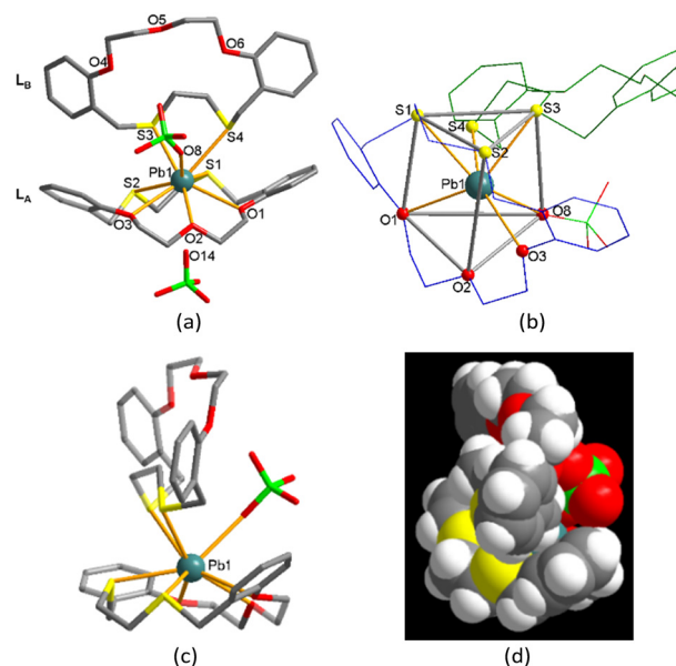
Fig. 1 An unsymmetrically sandwiched lead(II) complex, [\text{Pb}(\text{L})_2(\text{ClO}_4)]\text{ClO}_4 \cdot 0.5\text{CH}_2\text{Cl}_2 \cdot 0.5\text{CH}_3\text{CN} ( 1 ): (a) front view, (b) coordination environment of the lead(II) centre, showing a distorted di-capped trigonal prismatic geometry, (c) side view and (d) space-filling structure. Non-coordinated solvent molecules are omitted. Each non-coordinated perchlorate ion in (b–d) is not shown.
