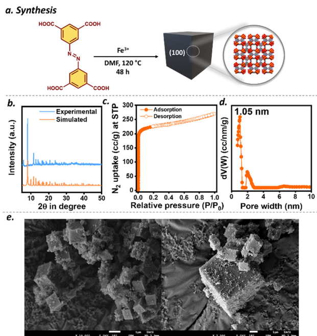
Fig. 1 (a) Schematic representation of the synthesis of Fe-soc-C, (b) simulated and experimental PXRD pattern, (c) \text{N}_2 adsorption–desorption isotherm, (d) pore size distribution plot and (e) FE-SEM images.
