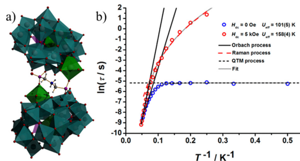
Fig. 8 The molecular structure (a) and magnetic relaxation plot (b) of [(\text{As-W}_9\text{O}_{33})_3\text{Dy}_2(\text{H}_2\text{O})_4\text{W}_4\text{O}_9(\text{H}_2\text{O})_2(\text{NH}_2(\text{CH}_2\text{PO}_3)_2)]^{33-} . Color code: cyan octahedron {WO 6 }, green polyhedral Dy unit, red O, blue N, pink P, grey C, white H. Hydrogen atoms are omitted for clarity. Figure reprinted (adapted) with permission from ref. 136. Copyright (2017) American Chemical Society.
