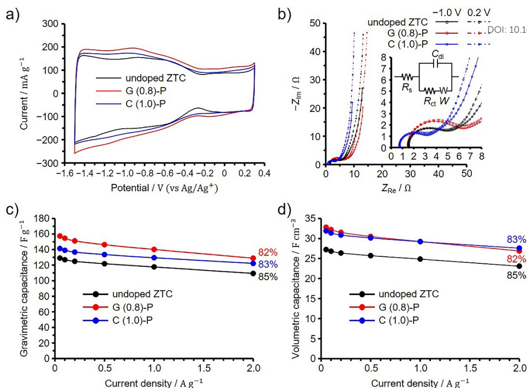
Fig. 4 Results of three-electrode cell measurements for G (0.8)-P and C (1.0)-P performed at 25 °C, shown alongside the results of the undoped ZTC. (a) Cyclic voltammogram collected at 1 mV s -1 . (b) Nyquist plots collected at -1.0 and 0.2 V (vs Ag/Ag + ). Insets show the magnified spectra at low frequencies and the equivalent circuit; R_s , R_{ct} , C_{dl} , and W represent series resistance, charge transfer resistance, double-layer capacitance, and Warburg impedance, respectively. 50, 51 (c, d) Dependence of (c) gravimetric and (d) volumetric capacitances on the current densities. Percentages in panels (c) and (d) indicate the capacitance retentions at 2 A g -1 based on the capacitances at 0.05 A g -1 .
