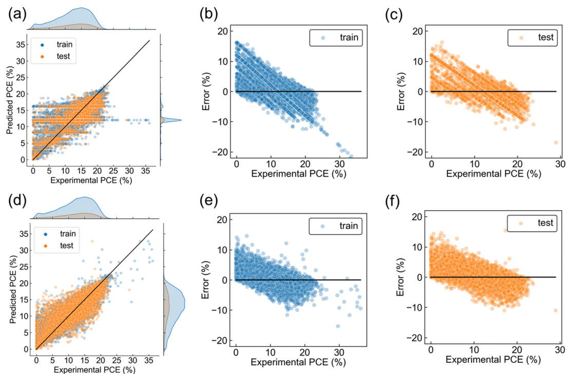
Fig. 4 Regression results and error analyses. (a) The joint plot of experimental-predicted plot and density plot when using only perovskite composition represented by Olynyk, and error plots of (b) training and (c) test. Error was defined as prediction minus experimental PCE. (d) The joint plot of experimental-predicted plot and density plot when using material and process information by the best representation, and error plots of (e) training and (f) test. In all panels, solid black line presents the reference line when predicted values are perfectly matched with experimental values.
