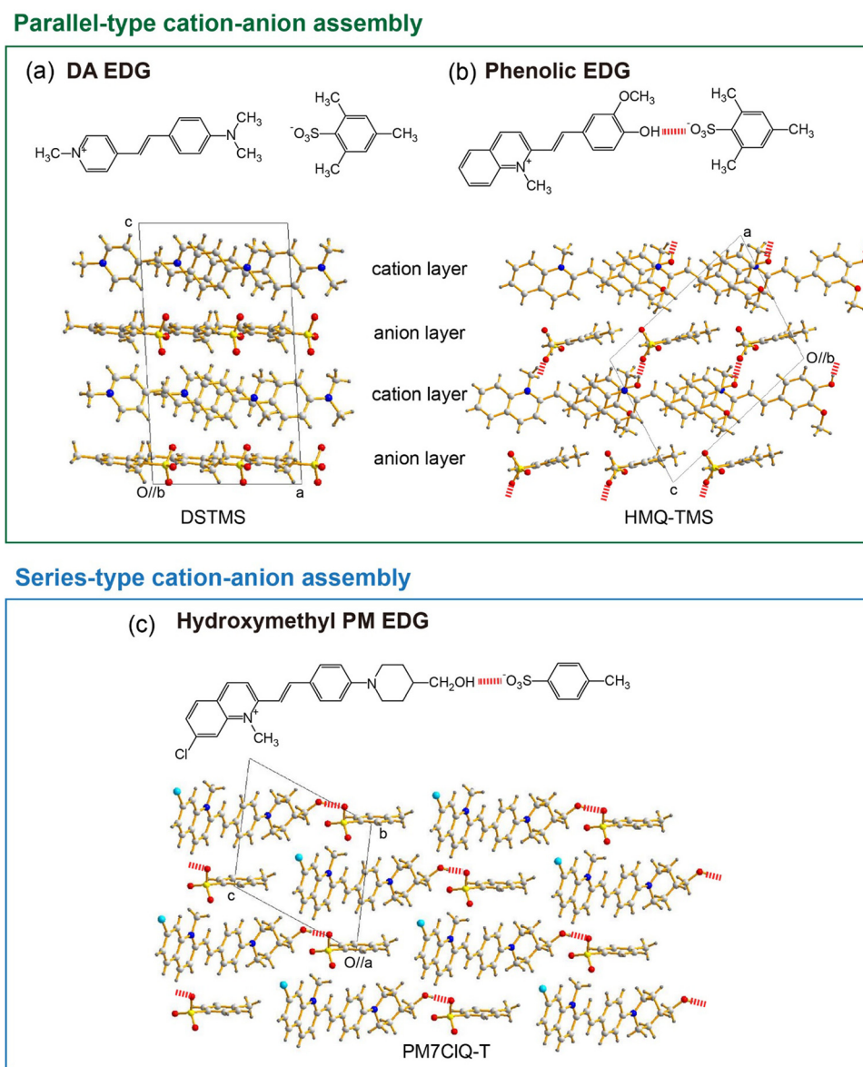
Fig. 3 Molecular ordering of ionic organic THz crystals: parallel-type cation–anion assembly with (a) DA EDG (DSTMS crystals here) and (b) phenolic EDG (HMQ-TMS crystals with HM EDG here) and (c) series-type cation–anion assembly with hydroxymethyl PM EDG (PM7CIQ-T crystals here).
