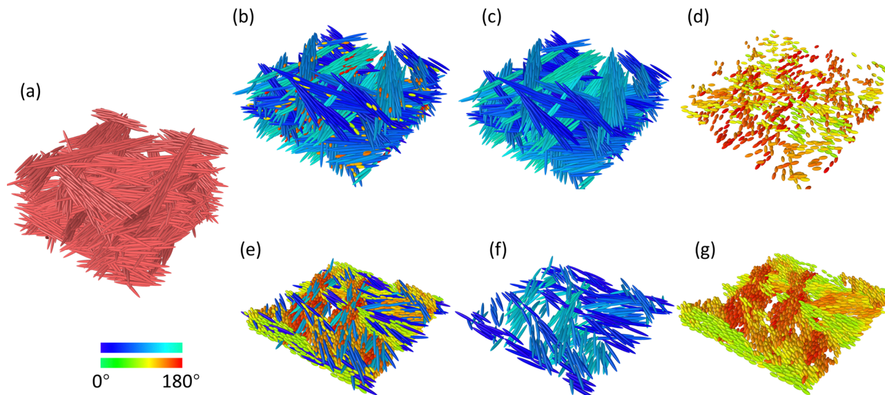
Fig. 7 Structure of co-assemblies: (a) pure CNCs, (b) CNCs : AuNRs : 10 : 1 and (e) 1 : 2. (c), (d), (f) and (g) represent the separated structure of CNCs and AuNRs respectively. The colour coding represents the angle between the elongation direction of the particles and the backplane.
