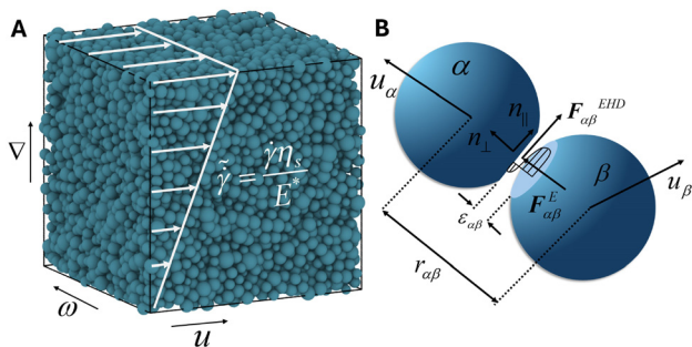
Fig. 1 (A) Configuration of suspensions with volume fraction of \phi = 0.80 in a cubic simulation box that is in the shear flow with an applied shear rate of \dot{\gamma} = \dot{\gamma} \eta_s / E^* , where E^* is the particle contact modulus and \eta_s is the suspending fluid viscosity. The flow ( \mathbf{u} ), gradient ( \nabla ), and vorticity ( \boldsymbol{\omega} = \nabla \times \mathbf{u} ) directions are shown. (B) Two particles form flat facet at a contact and interact via generalized Hertzian contact and elasto-hydrodynamic lubrication forces. 3
