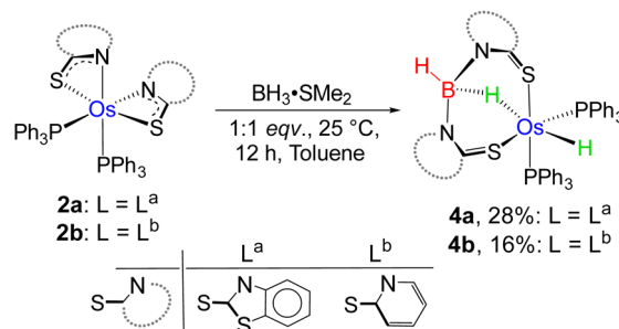
Scheme 2 B–H activation by \text{Os}(\text{II})\text{-N,S} -chelated complexes, 2a–b .
