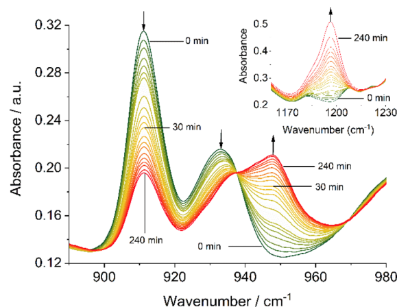
Fig. 4 Solution-IR spectra in the region of the \text{Mo}=\text{O} stretching bands ( 890\text{--}900\text{ cm}^{-1} ) of 3^{\text{C(O)OMe}} (50 mM in \text{DMF} ), 10 equivalents \text{PPh}_3 and 50 equivalents \text{DMSO-d}_6 in \text{DMF} irradiated at 410\text{ nm} as a function of time; insert— \text{O}=\text{P} stretching band ( 1160\text{--}1230\text{ cm}^{-1} ) of the same sample.
