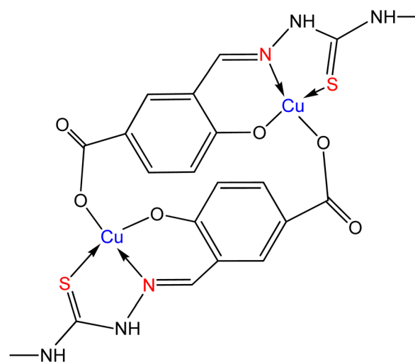
Fig. 18 Cu(II) complex of water-soluble thiosemicarbazone ligand.
