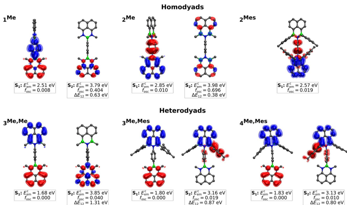
Fig. 4 Isosurface plots of the unrelaxed difference density (hole [red] and electron [blue]), calculated emission energies ( E_{\text{em}}^{\text{c}} ), and oscillator strengths ( f_{\text{osc}} ) in \text{CH}_2\text{Cl}_2 for the first two excited states of the homo- ( 1^{\text{Me}} , 2^{\text{Me}} , 2^{\text{Mes}} ) and heterodyads ( 3^{\text{Me,Me}} , 3^{\text{Me,Mes}} , 4^{\text{Me,Mes}} ) at the TDA-OT-LRC- \omega PBEh-D4/def2-TZVPP/SS-PCM[ \text{CH}_2\text{Cl}_2 ]/ \Delta SCF/UKS/PCM level of theory. 0.997 [opaque] and 0.999 [translucent] were used as isovalues. 45
