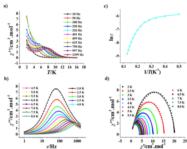
Fig. 6 Plots of \chi'' versus T for D-1 ( H_{\text{dc}} = 0 Oe). (a). Frequency dependence of \chi'' for D-1 at a zero dc field (b). Plot of \ln(\tau) versus 1/T for D-1 ( H_{\text{dc}} = 0 Oe); the solid line represents the best fitting with quantum tunnelling plus Orbach plus Raman (c). Cole–Cole plots measured from 2.0 to 8.0 K for D-1 ( H_{\text{dc}} = 0 Oe); the solid lines represent the best fitting with the generalized Debye model (d).
