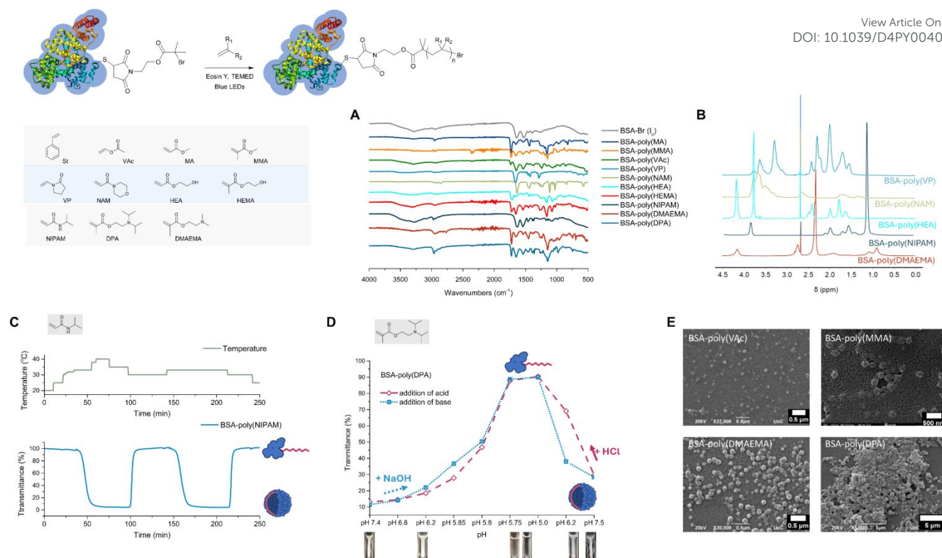
Figure 3. Characterization of amphiphilic, hydrophilic, and responsive protein-polymer conjugates. A. IR spectra of the bioconjugates. B. ^1\text{H} -NMR spectra acquired for hydrophilic BSA-polymer conjugates. C. Transmittance vs. time curve at different temperatures showing the rapid response of BSA-poly(NIPAM). D. Transmittance vs. pH curves of BSA-poly(DPA). Two cycles are shown for the same sample in which the response was induced by changing the pH with the addition of HCl (pH decrease) or NaOH (pH increase). E. SEM and FE-SEM micrographs of amphiphilic protein-polymer conjugate nanoparticles.
