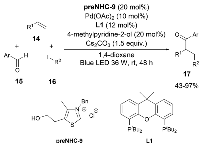
Scheme 9 Photoredox NHC/Pd synergistically catalysed alkylacylation of aldehydes.
