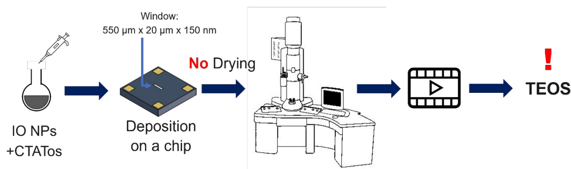
Scheme 3: Schematic representation of the procedure followed to perform the first in situ LPTM experiment.
