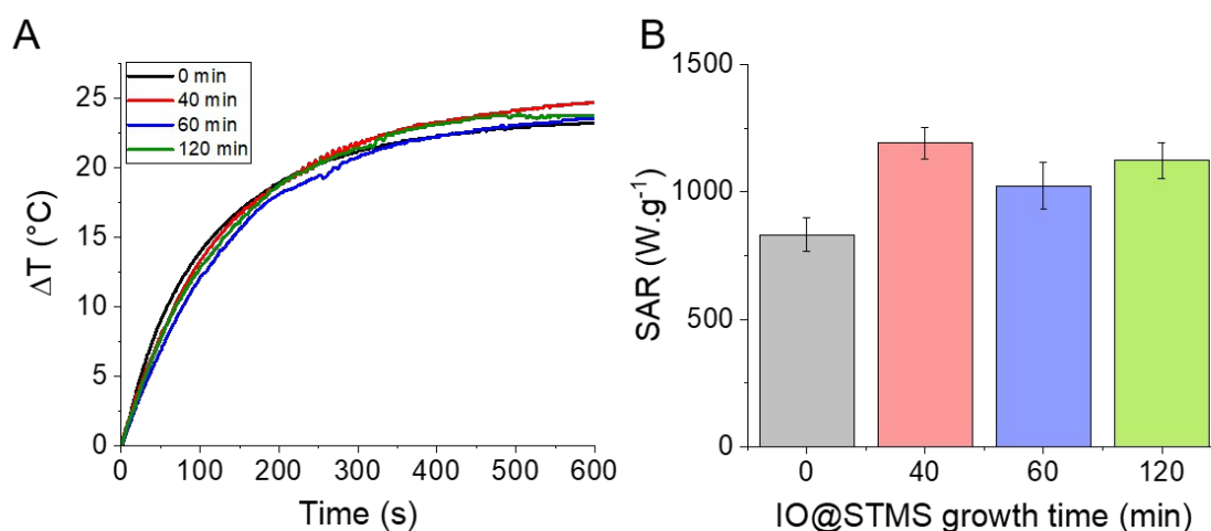
Figure 11: A) Temperature profiles as a function of time for the different IO@STMS-t NPs at 0.5 \text{ mgFe.mL}^{-1} under NIR light irradiation. B) Corresponding SAR values. These results were obtained with the IO@STMS-t obtained from series 2.
