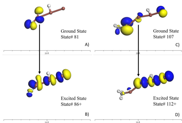
Fig. 4 TDDFT results for the F111 ( H_2FI_3 ) molecule (A and B) and C[I][I]I11 (C and D). Subfigure A and C illustrate the ground states local density of states surfaces. The yellow is associated with spin-up and blue is associated with spin-down electrons. Subfigure B and D are the excited states local density of states. Comparing the ground state to the excited states provide spatial information of the electron transition outlined in Table 1. It is desirable to have a high overlap of these states to avoid decoherence of the states.
