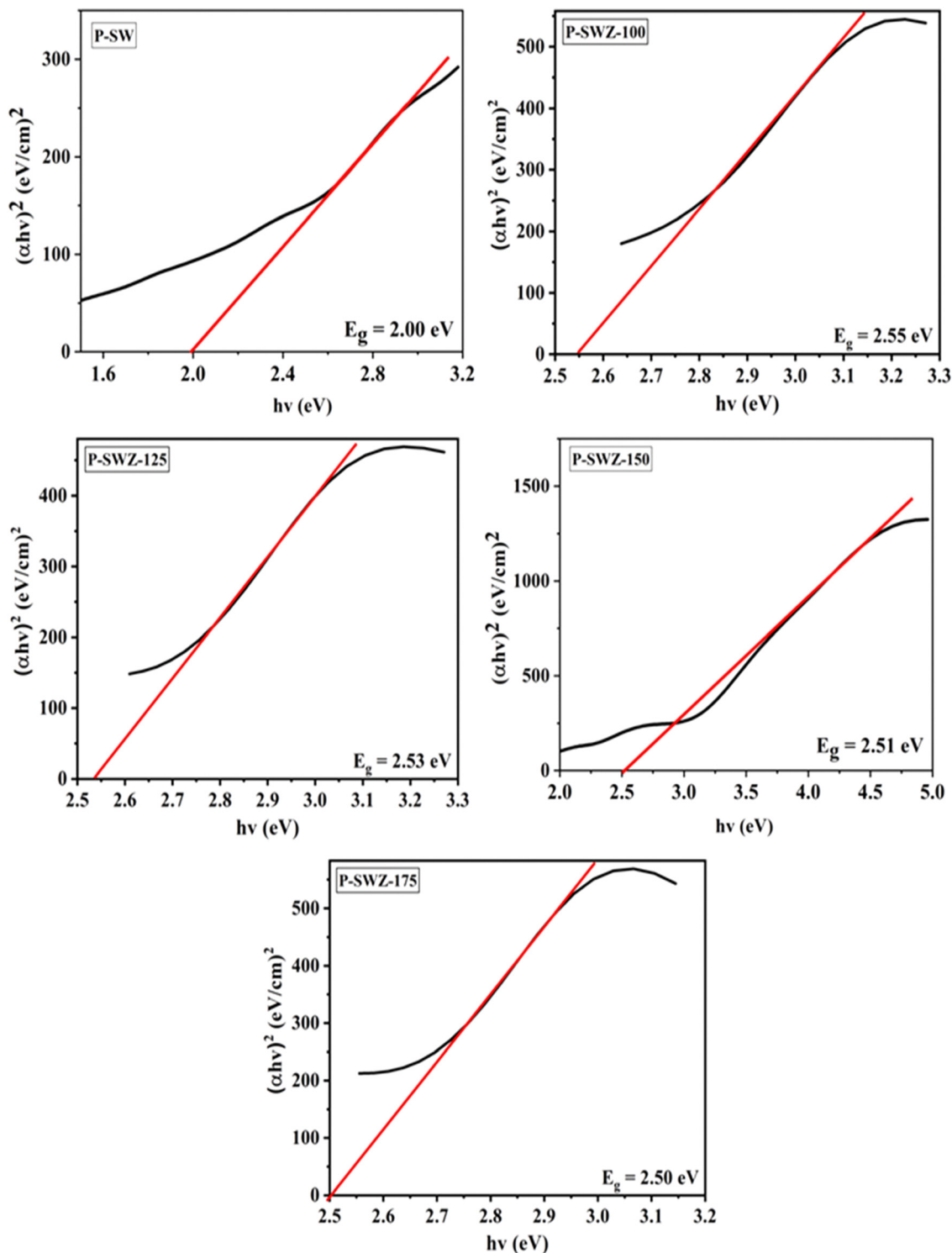
Fig. 8 Fitting energy band-gap of the SWCNT and SWCNT/ZnO NC integrated Si thin film.
