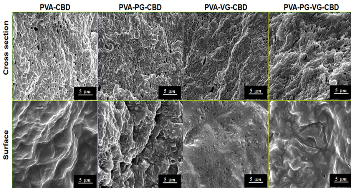
Fig. 2 SEM of CBD-rich hydrogels, showing that the interiors (cross sections) of the gels are sub microporous and the surface of the gels is nonporous. The addition of PG and VG can affect the pore size and porosity inside the materials, with the PVA-PG-VG showing the highest porosity.
