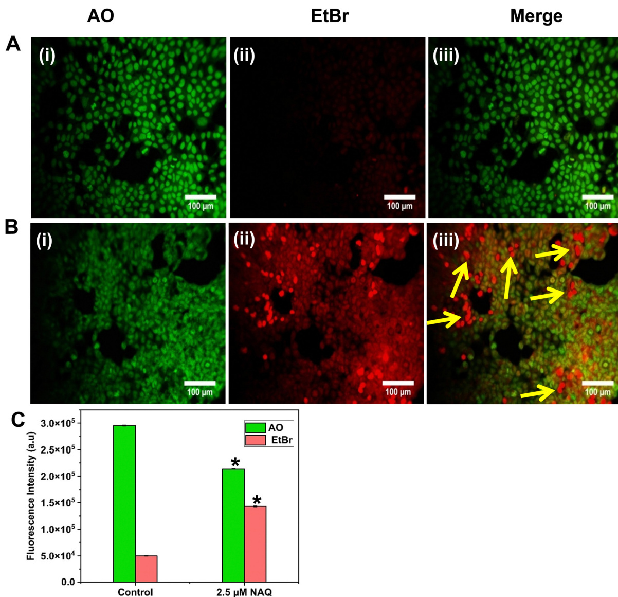
Fig. 8 Acridine orange (AO) and ethidium bromide (EtBr) staining of MCF-7 cells after 24 h of treatment with NAQ: (A) untreated cells. (B) NAQ ( 2.5 \mu\text{M} ) treated cells (yellow arrows indicate dead cells with the uptake of EtBr); (i) AO stained, (ii) EtBr stained, and (iii) merged image of cells stained with AO/EtBr. (C) Graph showing the fluorescence intensity of AO and EtBr. * denotes the significance level at P < 0.05 as compared to the control.
