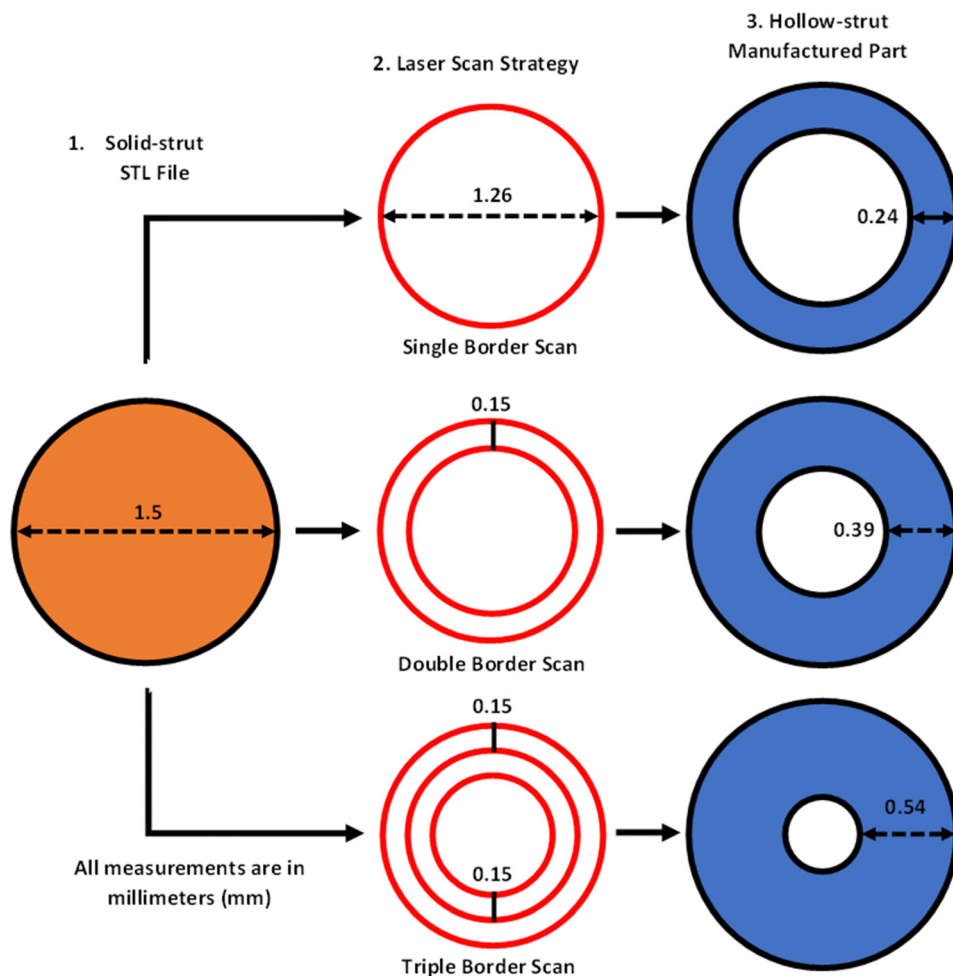
Fig. 2 LPBF of submillimeter hollow channels (schematic). Step 1: solid-strut STL file with the designed outer diameter (1.5 mm, orange). Step 2: formation of a hollow-strut geometry with different inner diameters or wall thicknesses through three laser scan strategies (red lines) including; single border scan (1B), double border scans (2B), and triple border scans (3B), where red is the scan path. Step 3: manufactured hollow strut cross-sections (blue).
