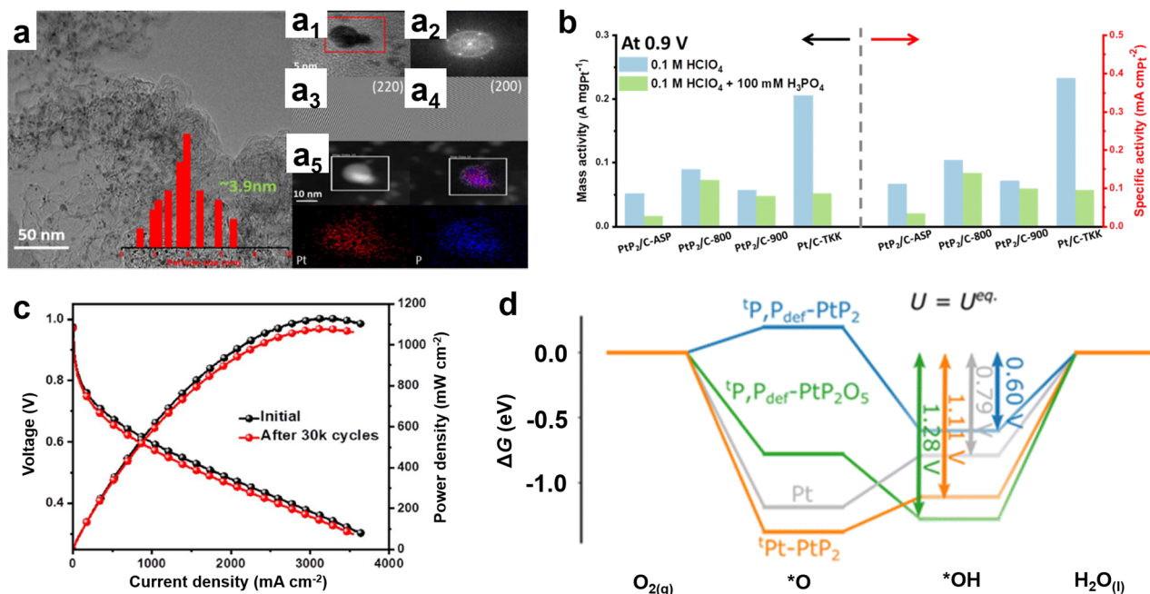
Fig. 9 (a) TEM image of PtP 2 /C-800 electrocatalysts, the inserted bar graph shows the PtP 2 particle size distribution along with the average PtP 2 particle size. (a1) HR-TEM image. (a2) FFT patterns of the area enclosed in the red square in (a1). (a5) HAADF images and the corresponding EDX images of (a1). (a3 and a4) Inverse FFT images of the area enclosed in the red square in (a1), where (a3) shows the distribution of 220 planes while (a4) shows the presence of 200 planes. (b) Mass and specific activity profiles; (c) long-term durability tests of PtP 2 /C-800; (d) free energy diagram for the ORR on four different active site models constructed from the (111) surfaces. Reprinted with permission from ref. 53. Copyright 2023, Royal Society of Chemistry.
