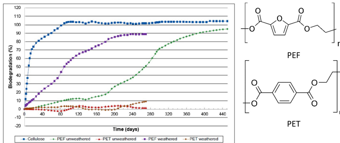
Fig. 8 Biodegradation profiles of weathered and un-weathered PEF, as well as weathered and un-weathered PET and cellulose as a reference material. Biodegradation (%) = amount of polymer converted to \text{CO}_2 (up to 450 days) with air/oxygen @ 58 °C in soil. All curves are the averages of three samples. 85
