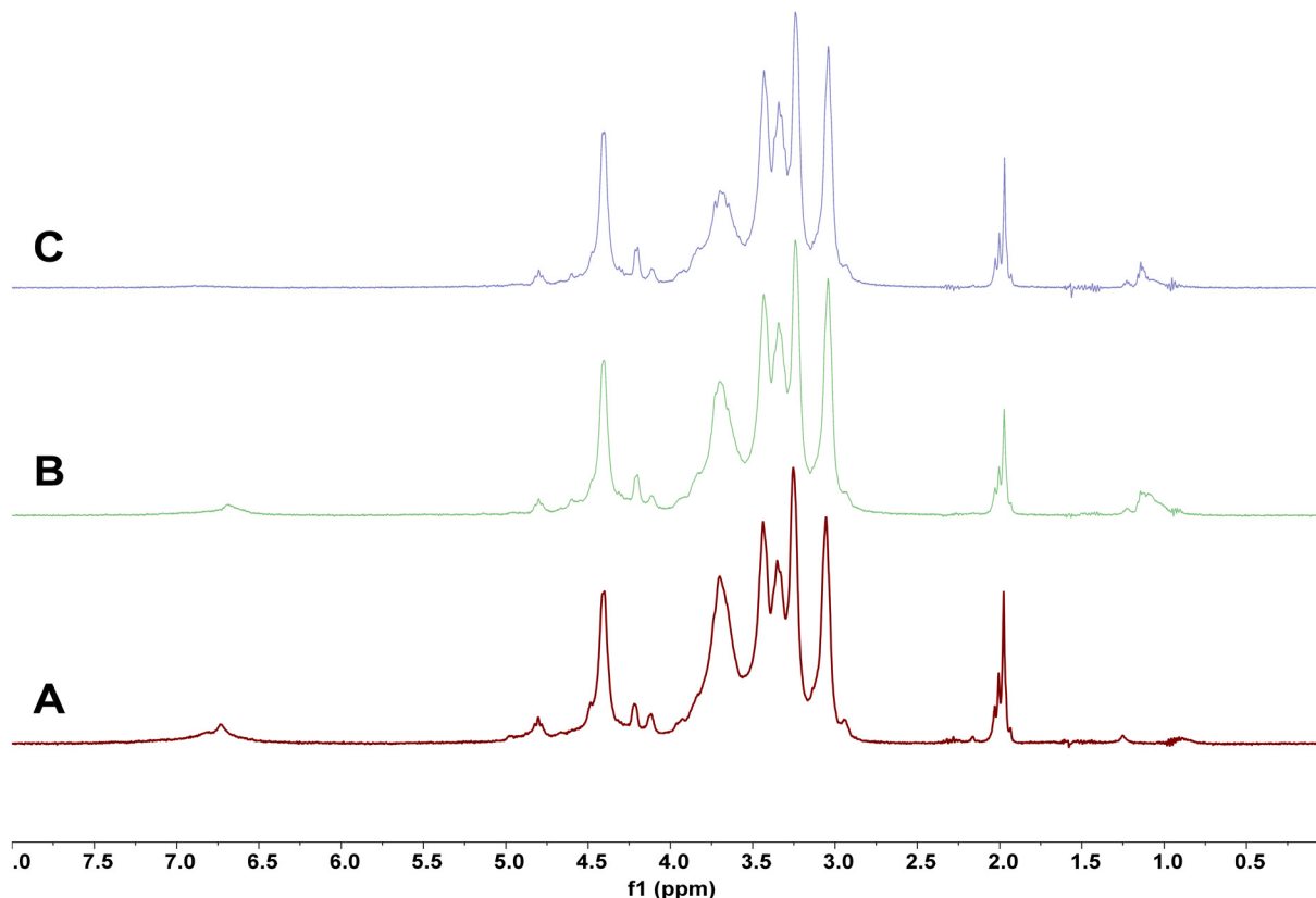
Fig. 5 Stack of diffusion edited ^1\text{H} spectra ( \text{P}_{4444}[\text{OAc}] : \text{DMSO-}d_6 , 1 : 4 wt%; 400 MHz; 65 °C) of cellulose-rich solids (measuring concentration 2.5 wt%) obtained on the RS of the S-500 control sample (A), RS after reactive extraction with the highest DS (conditions: [\text{EtOH}] = 99\% , [\text{H}_2\text{SO}_4] = 0.15 \text{ M} , t = 4 \text{ h} ) unbleached (B) and bleached (C). Despite the presence of insolubles in the measuring solutions, spectra A and B were not drastically different from previous reports on pulp samples obtained in used or similar electrolytes. Comparing spectra A and B it becomes evident that higher severity factors lead to the incorporation of ethoxy functionalities also in the polymeric fractions according to an additional peak at around 1 ppm characteristic of an ethoxy \text{CH}_3 moiety. After additional bleaching of the high severity HTT solid (C) the lignin fractions are effectively removed, while the ethoxy peak at least partly remains. This indicates that the modification partially occurred on the polysaccharide fractions of the RS, presumably on the hemicelluloses.
