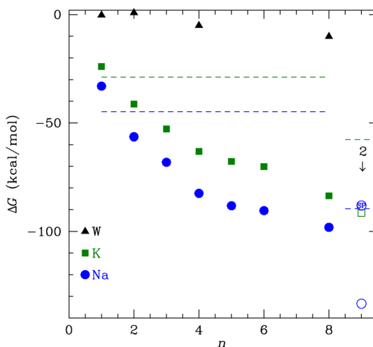
Fig. 2 \Delta G as a function of the number of NMA ligands, n , for K^+ , Na^+ and water (W). Horizontal dashed lines give the calculated free energy for ion hydration, which defines the reference state. The open points are for occupancy by two cations and the point with SP inside is from a single point calculation; see text for details.
