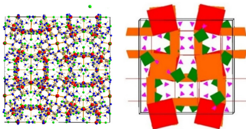
Fig. 3 Unit cell content in the cubic ( I\bar{4}3d ) structure of (\text{NH}_4)[(\text{InCl}_2)_3(\text{C}_{12}\text{N}_{20}\text{H}_8)]\cdot\frac{2}{3}[\text{InCl}_3(\text{NH}_3)] (left) and a schematic polyhedra drawing in the structure (right), emphasizing \text{NH}_4^+ ions as tetrahedra (violet) and [\text{InCl}_3(\text{NH}_3)] molecules as distorted octahedra (green).
