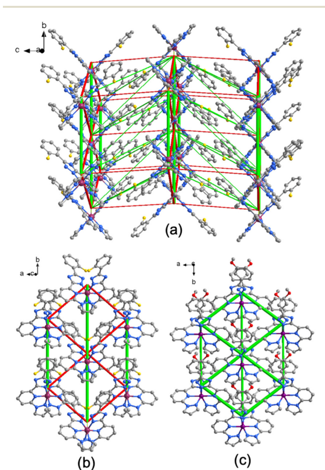
Fig. 5 (a) EDF of compound 2F , constructed using the values from the Table S5,† column “ \Delta E(\text{total})(\text{LS} - \text{HS}) ,” and superimposed on a fragment of the LS phase crystal lattice. The red cylinders correspond to weakening interactions, the green cylinders to the strengthening interactions. Tube size is scaled proportionally to the absolute value of the interaction energy, cut-off is 0.5 kJ mol -1 ; (b) and (c) comparison of EDFs within the supramolecular layer corresponding the compound 2F and 3MeO . Tube size scale is the same in both figures.
