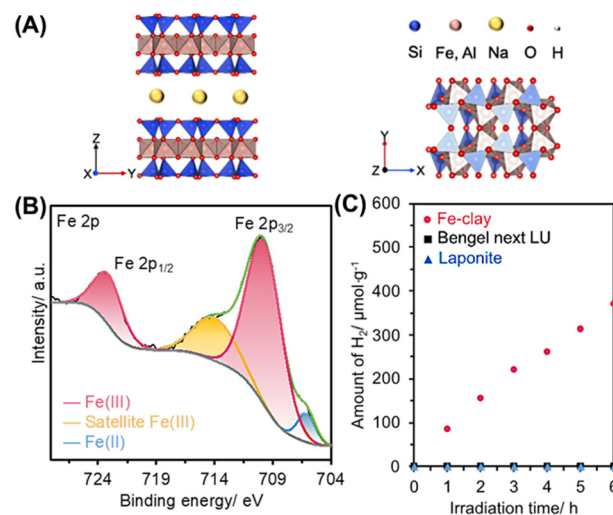
Fig. 20 (A) Polyhedral model of the smectite structure from the [100] direction and [001] direction, (B) Fe 2p XPS spectrum of Fe-clay, and (C) photocatalytic H 2 evolution of Fe-clay (red circle), Bengel next LU (black square), and LAPONITE® (blue triangle) from aqueous MeOH. 386
