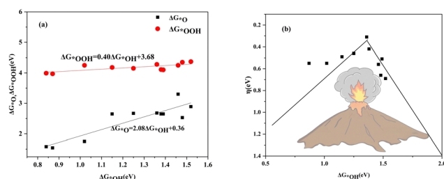
Fig. 13 (a) The scaling relationship of \Delta G_{*OOH} and \Delta G_{*OH} associated with \Delta G_{*OH} . (b) The volcano curve of the calculated \eta^{ORR} associated with \Delta G_{*OH} .
