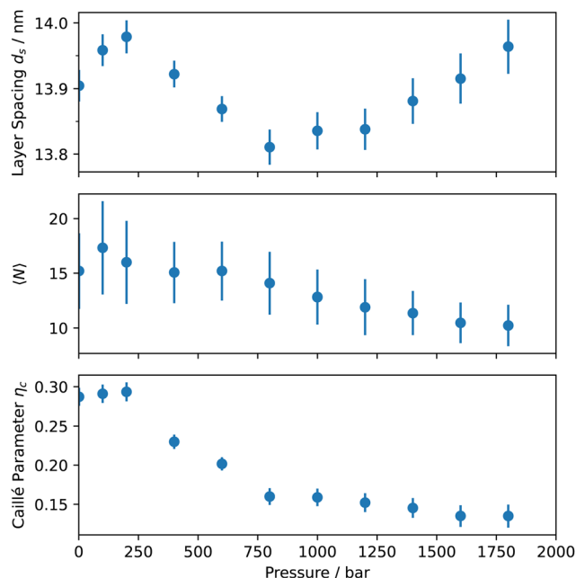
Fig. 3 Structural parameters obtained from the fit of the pressure dependent SANS data from \alpha CD- C_{12}E_5CH_2COONa complexes. From top to bottom: the interlayer spacing, the average number of aggregate involved in one multilayered aggregate, and the Caillé parameter, related to the membrane stiffness. Error bars result from the uncertainty determined from the least squares minimization procedure.
