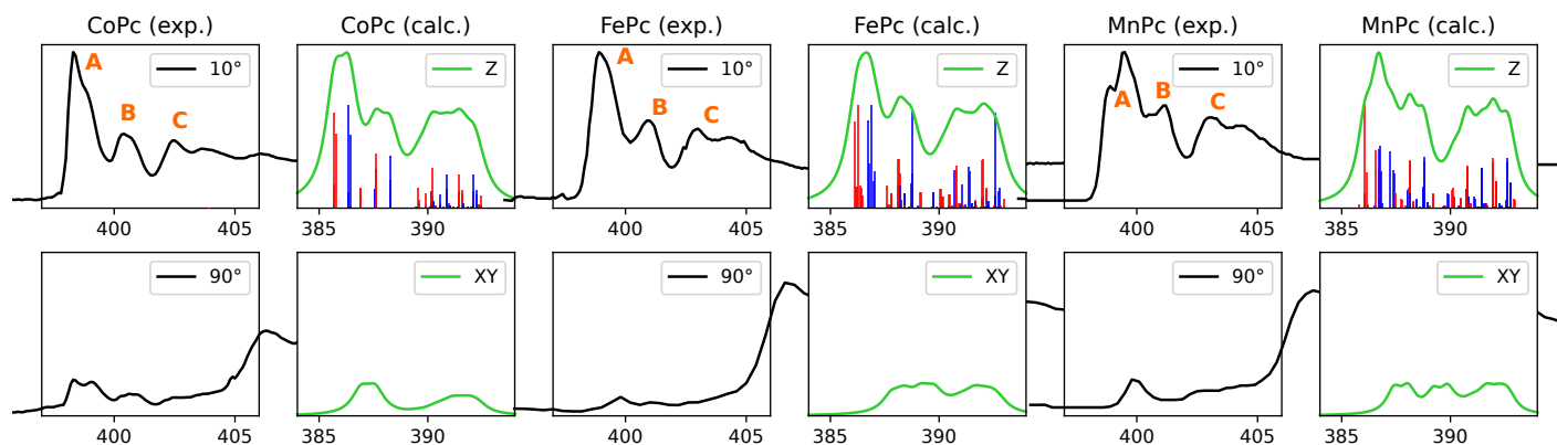
Fig. 6 Experimental (black) and calculated (green) nitrogen K-edge XAS for TMPcs. Energies are given in electronvolts, and the intensities are normalized. (The {}^2A_{1g} state of CoPc could only be located when a restricted open-shell Kohn-Sham (ROKS) wavefunction is employed, and these orbitals were fed into the TDDFT calculations without further iterations.)
