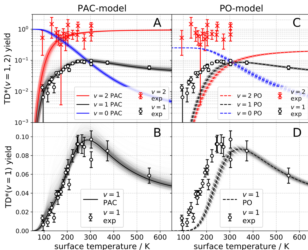
Fig. 6 Vibrational state-specific yields of desorbing molecules. (A)–(D) Experimentally observed CO ( \nu = 1 ) (open circles) and CO ( \nu = 2 ) (x symbols) passing through the TD* channel. The error bars indicate a 90% confidence interval. The black and red solid lines are the results of fits to the PAC model. (A) Logarithmic scale. (B) Linear scale. The black and red dashed lines represent the PO model. (C) Logarithmic scale. (D) Linear scale. The blue solid line (PAC) and the blue dashed line (PO) represent the desorbing yield of CO ( \nu = 0 ) stemming from the ultimate vibrational relaxation of CO ( \nu = 2 ). The shading represents the uncertainty of the fit. 74 From ref. 74 with permission from American Association for the Advancement of Science (AAAS) Copyright (2020).
