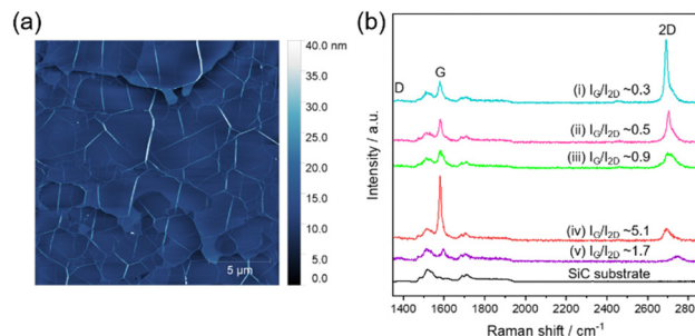
Fig. 2 (a) Topographic AFM image of TAGr grown on a SiC(0001) substrate. (b) Raman spectra of the TAGr and SiC(0001) substrate. Each spectrum was measured at different points in the same sample.
