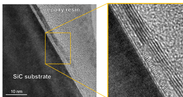
Fig. 1 Cross-sectional TEM image of a TAGr on SiC (0001).
