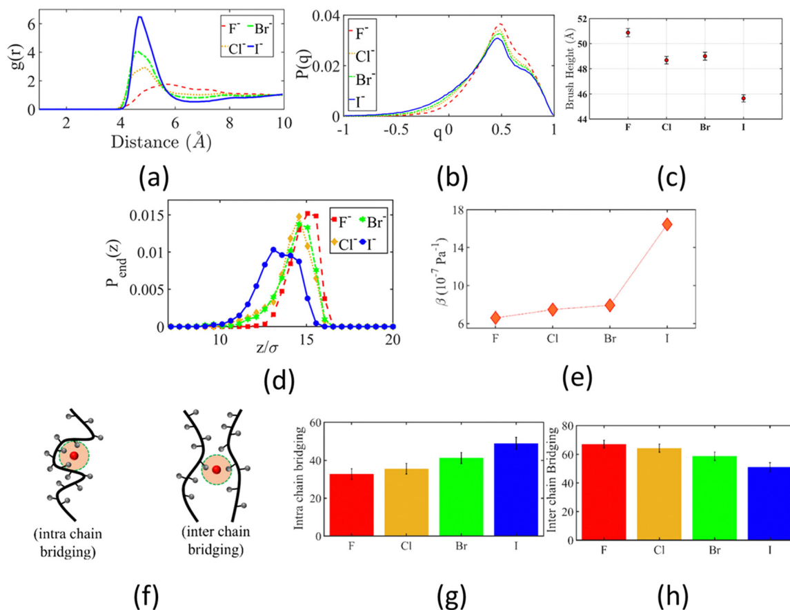
Fig. 24 (a) RDF of \{N(\text{CH}_3)_3\}^+ \text{-X} ( X = \text{I}^- , \text{Br}^- , \text{Cl}^- , and \text{F}^- ). (b) Probability distribution of the tetrahedral order parameter ( q ) of the solvating water of the \{N(\text{CH}_3)_3\}^+ moiety. (c) Variation of the height of the PMETA + brushes for the cases where the PMETA + brushes are screened by different halide counterions. (d) End chain monomer distributions of the PMETA + brushes. (e) Variation of the compressibility factor of the PMETA + brush system. In (b), (d), and (e), results are shown for the individual cases where the PMETA + brushes are screened by different halide counterions. (f) Schematic of two types of bridging interactions: intrachain bridging and interchain bridging. (g) Percentage of intrachain bridging undergone by the monomers of the PMETA + chains screened by different halide counterions. (h) Percentage of interchain bridging undergone by the monomers of the PMETA + chains screened by different halide counterions. All the parts of the figure have been reprinted with permission from Ishraq, R.; Das, S., All-Atom molecular dynamics simulations of cationic polyelectrolyte brushes in the presence of halide counterions, Macromolecules , 2024, 57 (7), 3037–3046. Copyright (2024) American Chemical Society.
