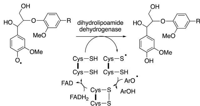
Fig. 11 Mechanism of phenoxy radical trapping by FAD-dependent dihydroliipoamide dehydrogenase containing an active site disulfide. ArOH represents a second 1-electron reduction of a phenoxy radical to a phenol.
