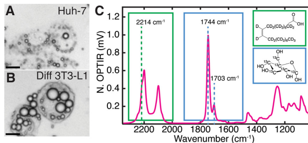
Fig. 2 Live cell characterization of the cell lines (A) Huh-7 and (B) differentiated 3T3-L1 after feeding with ^2\text{H} oleic acid (60 \mu\text{M} ) and ^{13}\text{C} glucose (4.5 \text{mg mL}^{-1} ). Scale bars are 20 \mu\text{m} . (C) Full IR spectra of a point within a fixed Huh-7 cell LD 48 hours after feeding ^2\text{H} OA. ^2\text{H} -C from the ^2\text{H} oleic acid (green, structure in inset) which has been esterified in LDs. 2214\text{ cm}^{-1} is assigned to ^2\text{H} -C stretching. ^{13}\text{C}=\text{O} stretch at 1703\text{ cm}^{-1} where the ^{13}\text{C} comes from metabolized ^{13}\text{C} glucose (blue, structure in inset). Pictured alongside the unlabelled ^{12}\text{C}=\text{O} band at 1744\text{ cm}^{-1} .
