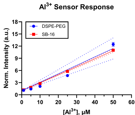
Fig. 2 Response of the \text{Al}^{3+} sensors made with DSPE-PEG and SB-16 to analyte ranging from 1 \mu\text{M} to 50 \mu\text{M} . While there is a small variation, both responses show a similar trend (two-tailed t -test, 95% C.I., p = 0.1134 > 0.05 ). Note, the data was normalized to the response at 1 \mu\text{M} , also where not visible the errors bars are smaller than the data points ( n = 3 ).
