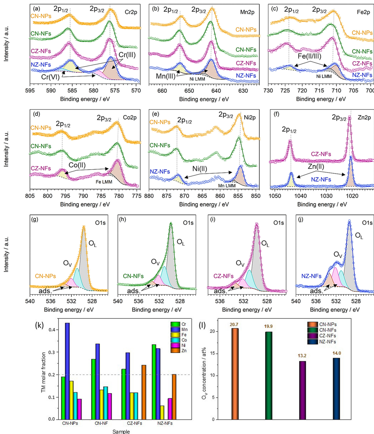
Fig. 3 High-resolution XPS spectra and fitting of (a) Cr 2p, (b) Mn 2p, (c) Fe 2p, (d) Co 2p, (e) Ni 2p, (f) Zn 2p and (g–j) O 1s core levels and resulting (k) TM molar fraction in the combination ( Cr_{0.2}Mn_{0.2}Fe_{0.2}M'_{0.2}M''_{0.2} ), where M'M'' denotes the metal pairs CoNi, CoZn and NiZn, and (l) O_V concentration. Labels indicate the peak assignment: O_V = oxygen vacancies; O_L = lattice oxygens; ads. = adsorbed or chemisorbed oxygen species (e.g., O_2 or H_2O ).
