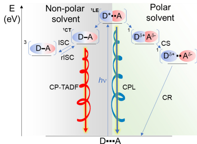
considering that only single-bond rotations are necessary to convert the folded conformers into their extended forms, and considering the fact that the systems contain excess energy following the photon absorption, the energy barriers associated with these bond rotations might be easily overcome, 53 and there are likely multiple pathways available for the compounds to reach one of the excited state potential energy minima. A broader exploration of the S_1 potential energy surface as well as the explicit treatment of solvent molecules aided by molecular dynamics simulations, 31 may clarify the molecular details underlying the mechanism of these processes, but such calculations are beyond the scope of the present study. The calculated dipole moments of the different conformers also reflect the stabilization that benefits the extended and folded structures in the two solvents, especially in the excited state. The extended conformers exhibit the highest dipole moments in the ground state, the folded conformers exhibit the lowest dipole moments, and the partially folded structures have intermediate values (see ESI, † Table S29). Given how energetically close the different conformers are, it is likely that the higher-energy conformers 3a and 4b , responsible for the negative CPL, become accessible in the more polar solvent DCM, whereas the folded conformers that yield a positive CPL remain predominant in the less polar MCH. It should also be noted that the folded structures potentially form non-luminescent exciplexes in the more polar solvent, as sketched schematically in Scheme 2 ( vide infra ). This statement, and our conclusions derived from calculations are consistent with previous reports, 54–57 involving donor–acceptor units linked together by methylene chains [(CH_2)_n] , n = 3 for the molecules studied here], where different conformers of the same compounds were found to be responsible for different emission profiles depending on the solvent polarity. For example, Majima and coworkers found that for linked donor–acceptor units based on naphthalimide and phenothiazine, polar solvents stabilize extended
