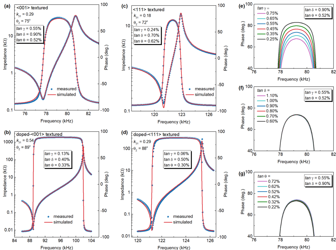
Fig. 5 Impedance and phase angle spectra for (a) <001> textured and (b) doped-<001> textured ceramics. Impedance and phase angle spectra for (c) <111> textured and (d) doped-<111> textured ceramics (the mechanical loss \tan \gamma , dielectric loss \tan \delta , and piezoelectric loss \tan \theta were fitted using loss incorporated equivalent circuit). (e)–(g) Simulated phase angle spectra for <001> textured ceramic with different loss factors.
