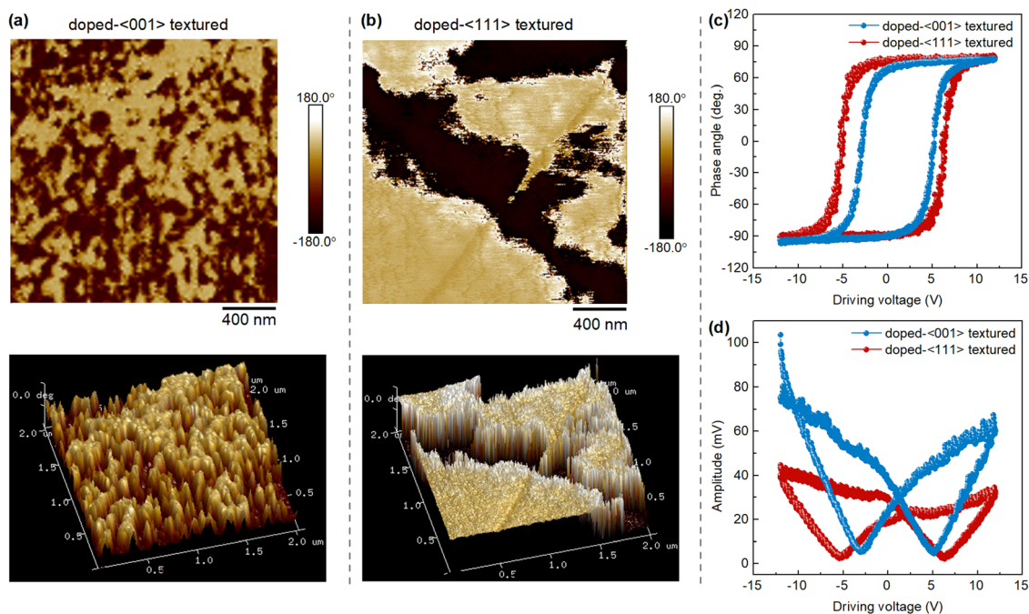
Fig. 6 (a) and (b) 2D and 3D PFM phase images of domain structure for doped-<001> and <111> textured ceramics. (c) Microscopic piezoresponse hysteresis loops and (d) butterfly-shaped amplitude versus driving voltage curves for doped-<001> and <111> textured ceramics.
