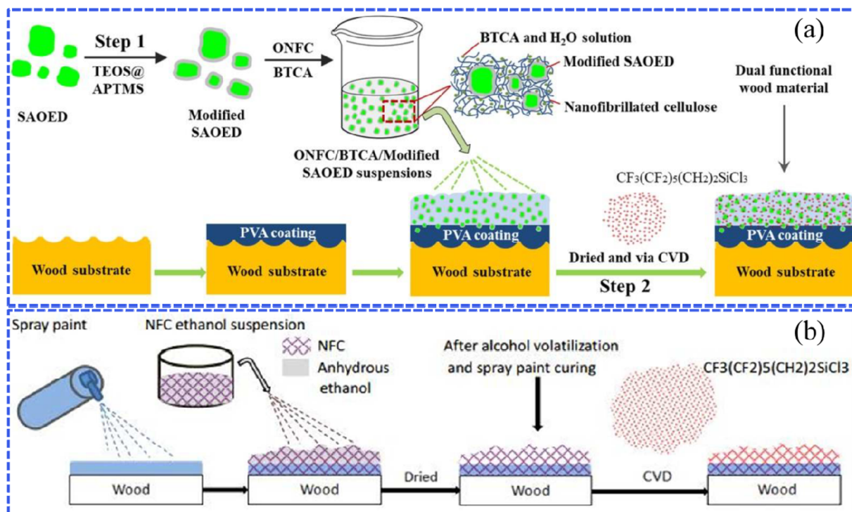
Fig. 3 (a) Schematic diagram showing the preparation of bifunctional wood that possesses superhydrophobic and fluorescence properties, which was treated with the modified SrAl 2 O 4 ·Eu 2+ Dy 3+ SAOED phosphor. Reproduced with permission from ref. 47. Copyright 2018, Elsevier. (b) A sketch of the preparation procedure for superhydrophobic nanofibrillated cellulose (NFC) coatings via the chemical vapor deposition (CVD) method. Reproduced with permission from ref. 48. Copyright 2016, Royal Society of Chemistry.
