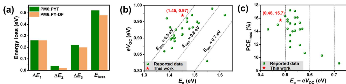
Fig. 5 (a) E_{loss} and its detailed three part values ( \Delta E_1 , \Delta E_2 , and \Delta E_3 ) of PM6:PYT and PM6:PY-DF-based devices. (b) Plots of eV_{OC} against E_g^{PV} and (c) PCE against E_g - eV_{OC} in all-PSCs with PCEs of over 9% reported in the literature.
