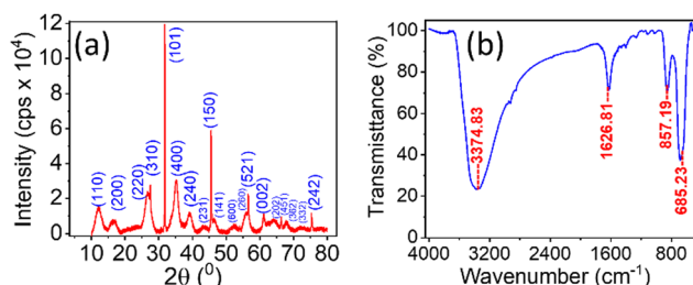
Fig. 2 (a) Powder XRD of NRs; the peaks resemble \beta -FeOOH (OH) with PDF card No. 01-079-5284. (b) FTIR transmission spectra in the KBr disk method for the NRs.
