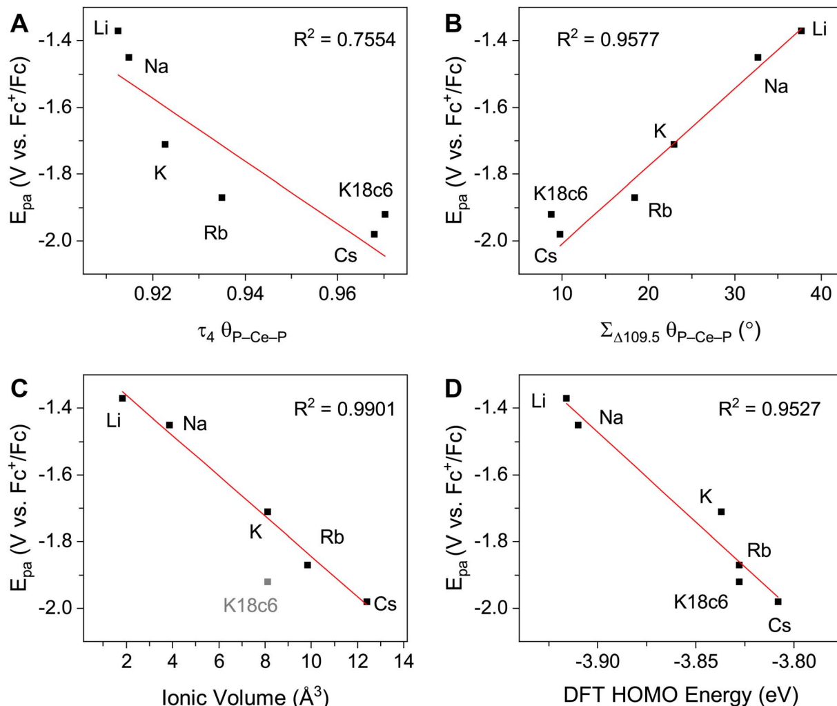
Fig. 3 E_{pa} measured by cyclic voltammetry (50 mM [^n\text{Bu}_4\text{N}][\text{BPh}_4] in THF) plotted vs. (A) \tau_4 calculated using P–Ce–P angles. (B) \Sigma_{\Delta 109.5} calculated using P–Ce–P angles. (C) Ionic volume ( 4/3 \cdot \pi r^3 , r = Shannon ionic radius 39 ), 2-Ce K18c6 data excluded from linear regression analysis. (D) Computed HOMO energy levels.
